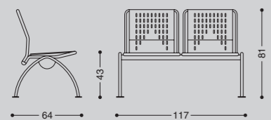
● 902B G/W/S/E/R/Y/A
