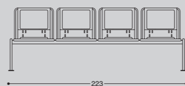
● 924B G/W/S/E/R/Y/A
