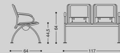
● 962B G/W/S/E/R/Y/A
