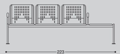
● 943BT G/T/W/T/S/T/E/T/R/T/Y/T/A/T
