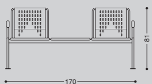
● 942BT G/T/W/T/S/T/E/T/R/T/Y/T/A/T
